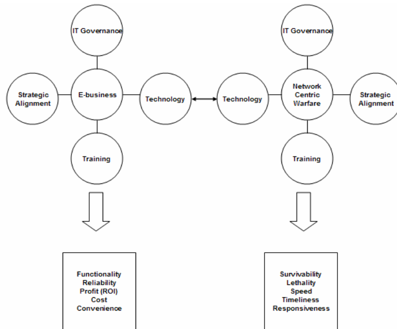
Figure 1: Proposed Model
