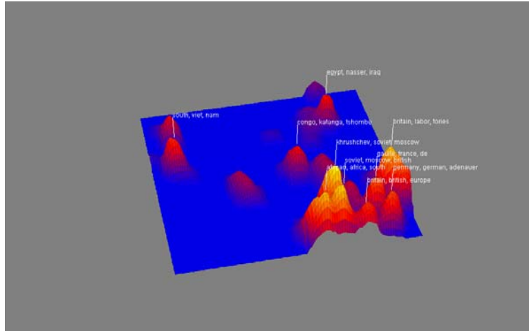
Figure 10: IN-SPIRE™ ThemeView
